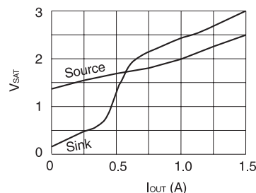
Saturation Curves
