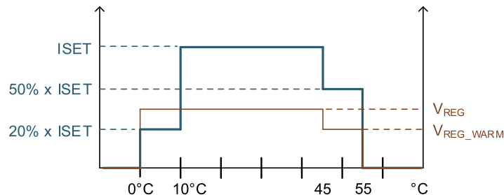
Figure 7-3. Standard JEITA Profile figure
