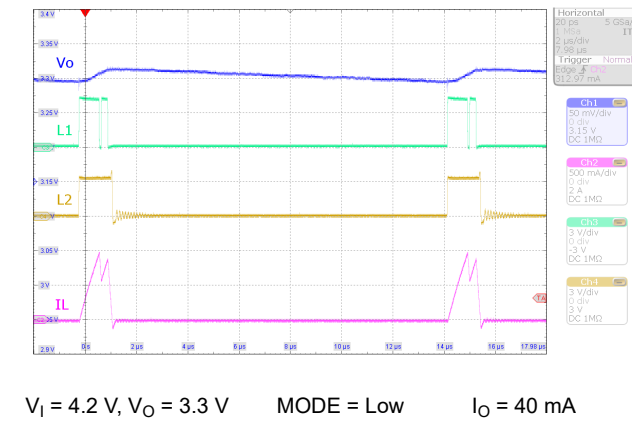
Figure 10-17. Switching Waveforms, PFM Buck-Boost Operation
