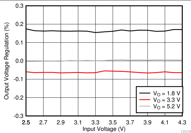
Figure 10-13. Line Regulation (PWM Only)
