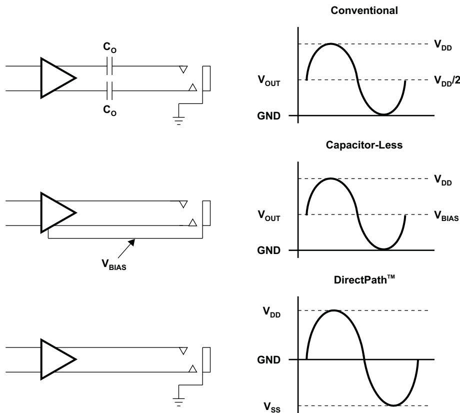
Figure 37. Amplifier Applications
