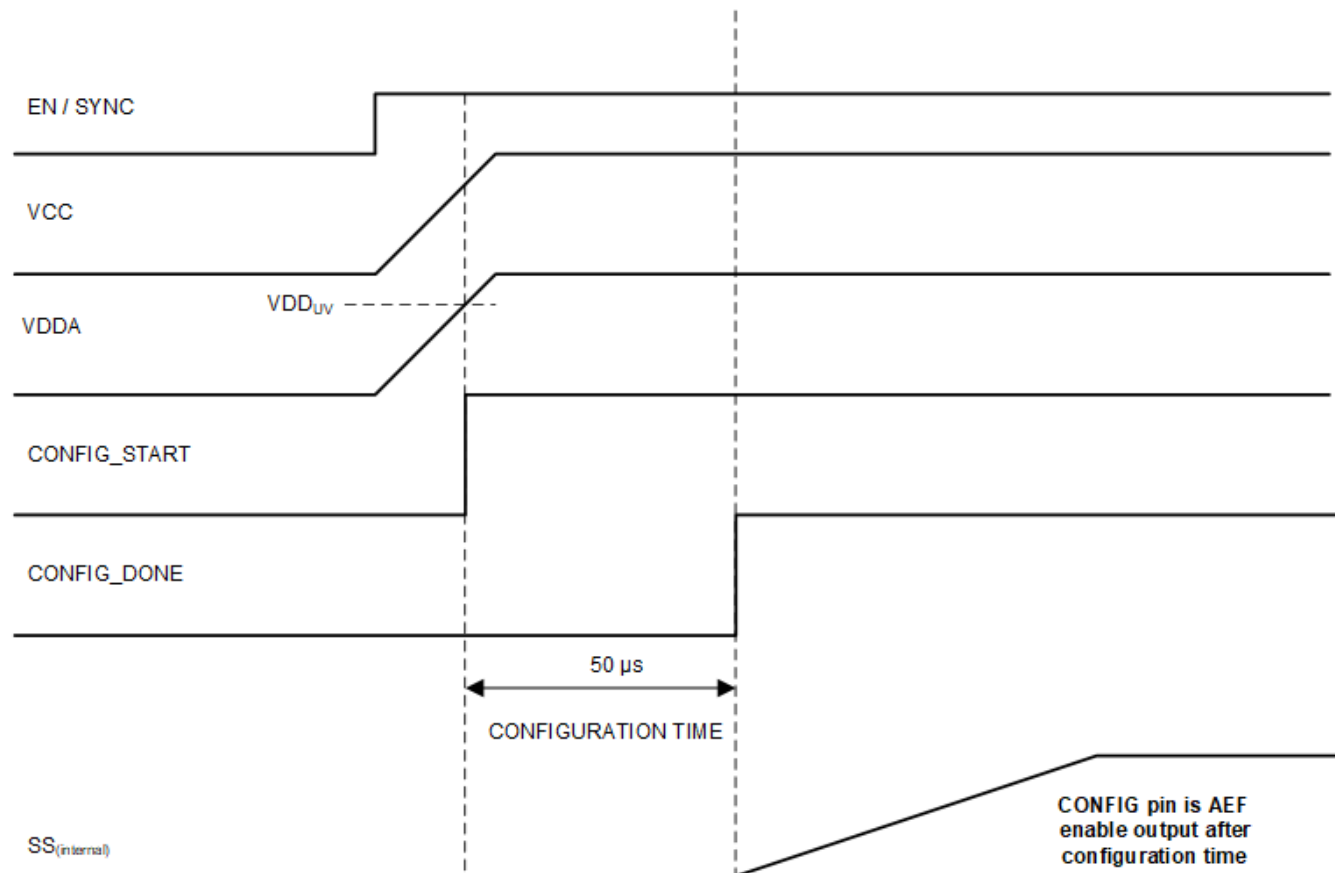
Figure 8-7. Configuration Timing
