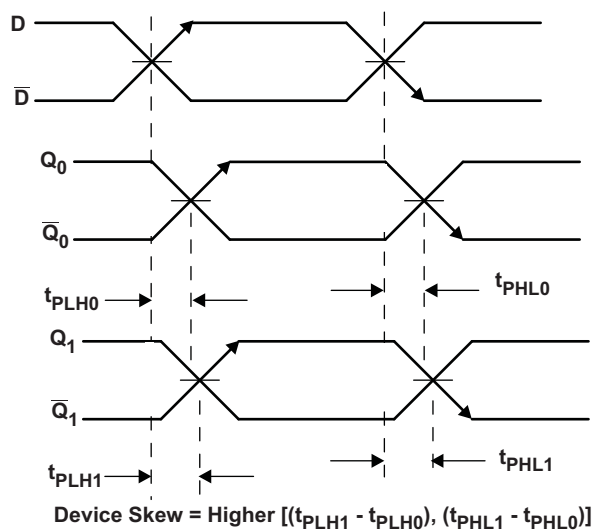
Figure 5. Device Skew
