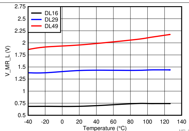
Figure 29. Manual Reset Logic Low Voltage Threshold Over Temperature for TPS3840DL-Q1
