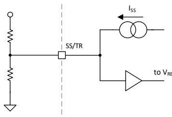
Figure 8-4. Tracking Operation Simplified Schematic
