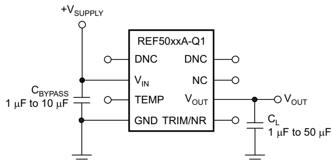
Figure 28. Basic Connections
