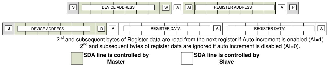
Figure 24. I²C Read Procedure
