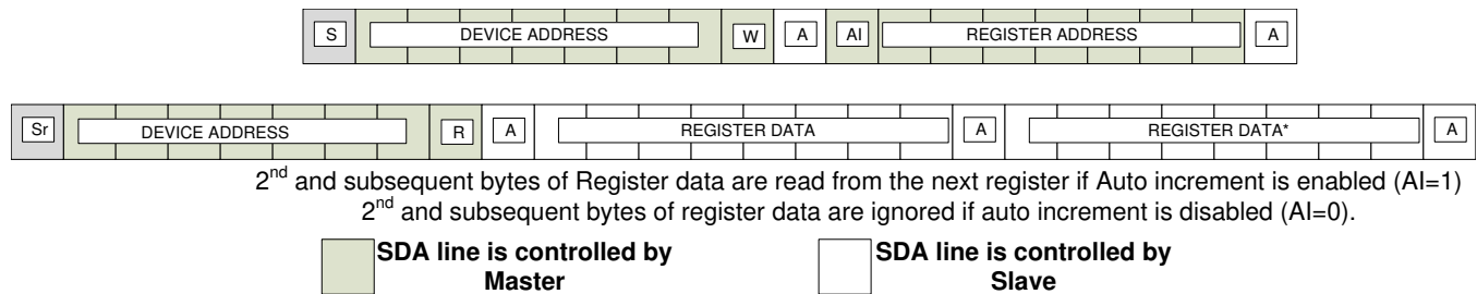
Figure 25. I²C Read Procedure with Repeated Start
