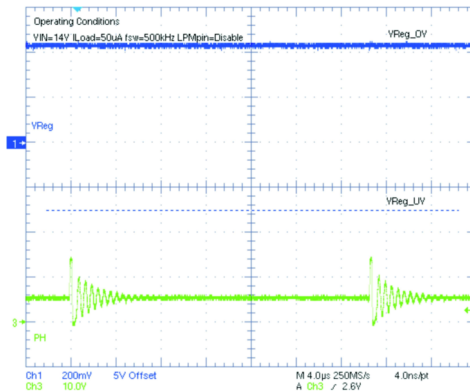
Figure 22. PSM at Nominal VIN
