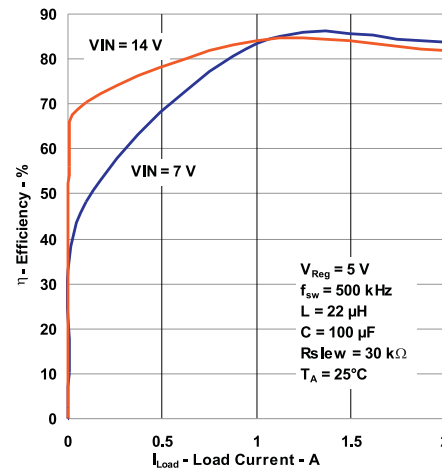
Figure 28. Efficiency vs Load Current for Different VIN
