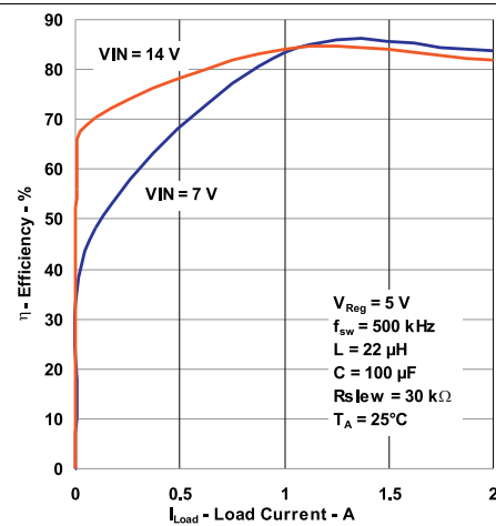
Figure 2. Efficiency vs Load Current for Different Vin
