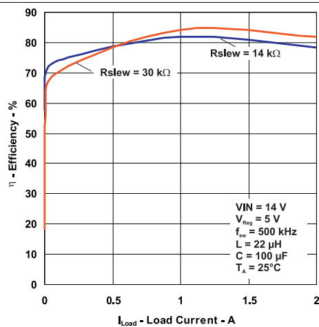
Figure 1. Efficiency vs Load Current for Different Rslew Resistors
