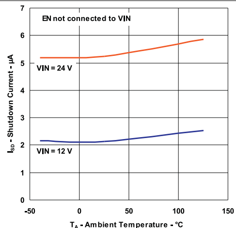
Figure 4. Shutdown Current Variation With Temperature
