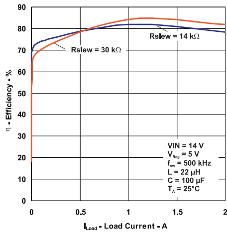
Figure 27. Efficiency vs Load Current for Different Rslw Resistors
