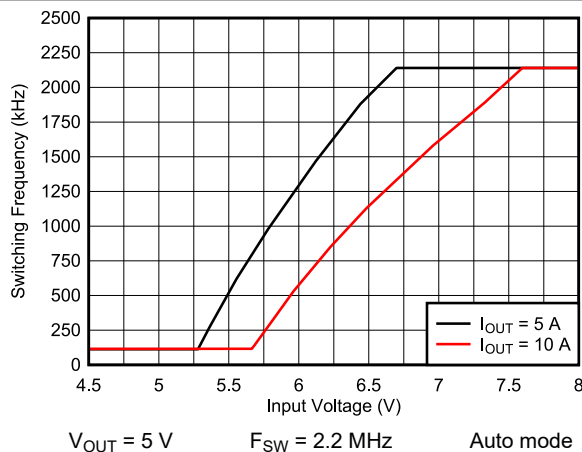
Figure 9-27. Frequency Dropout
