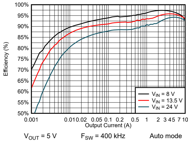
Figure 9-5. Efficiency
