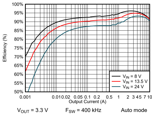
Figure 9-7. Efficiency
