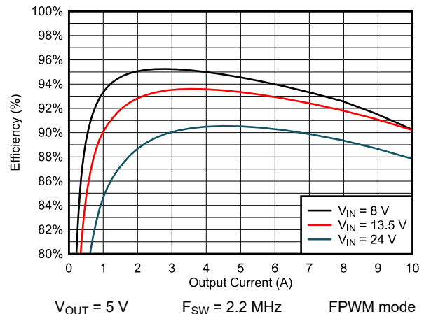
Figure 9-10. Efficiency
