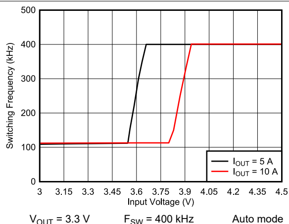
Figure 9-26. Frequency Dropout
