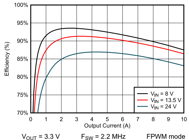
Figure 9-12. Efficiency
