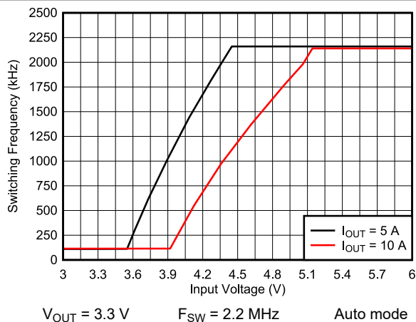
Figure 9-28. Frequency Dropout
