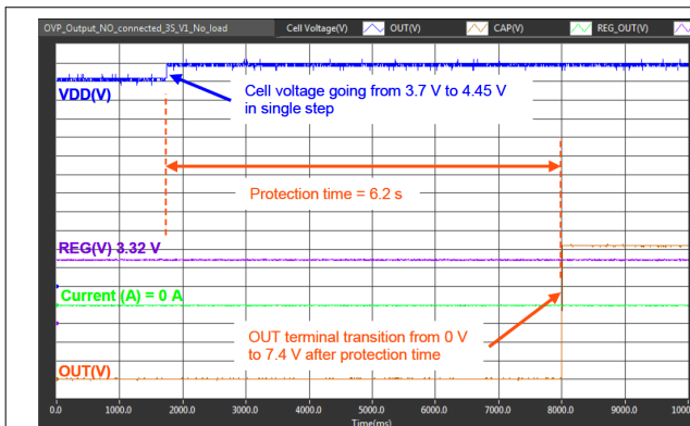
Figure 8-4. Overvoltage Protection
