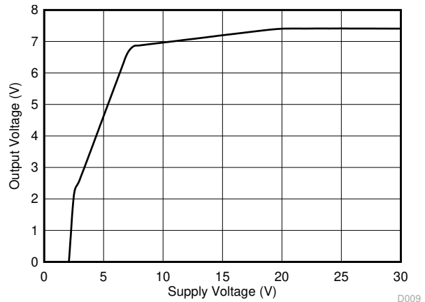
Figure 6-8. V_{OUT} vs V_{DD}
