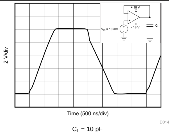
Figure 18. Large-Signal Step Response
