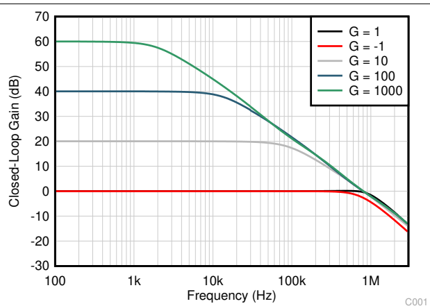
Figure 6-8. Closed-Loop Gain and Phase vs Frequency
