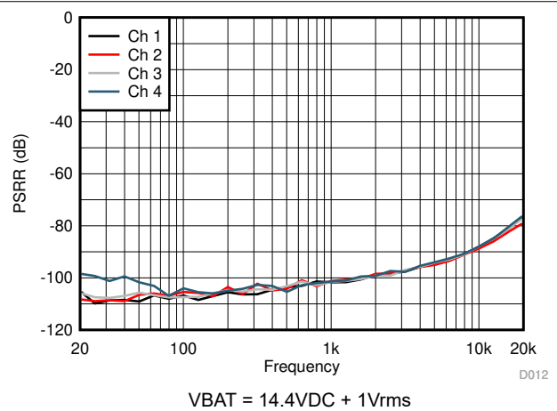
Figure 5-12. VBAT PSRR vs Frequency
