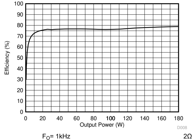
Figure 5-8. Efficiency vs Output Power
