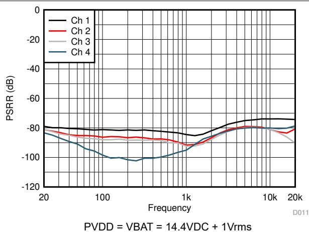
Figure 5-11. PVDD + VBAT PSRR vs Frequency
