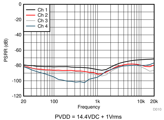
Figure 5-10. PVDD PSRR vs Frequency
