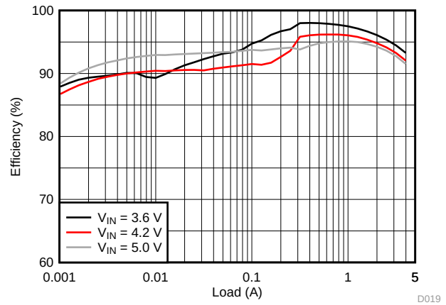
Figure 9. Efficiency, V_{OUT} = 1.2\text{ V}
