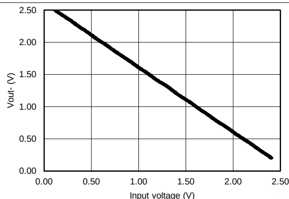
Figure 39. V_{OUT-} vs Input Voltage
