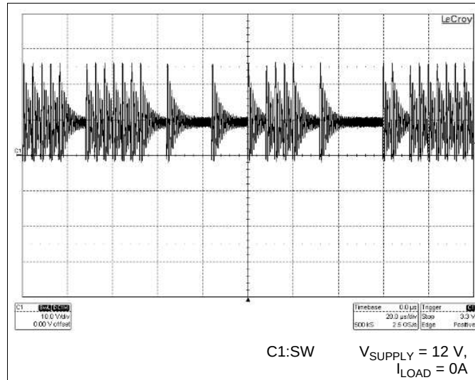
Figure 44. Pulse Skip
