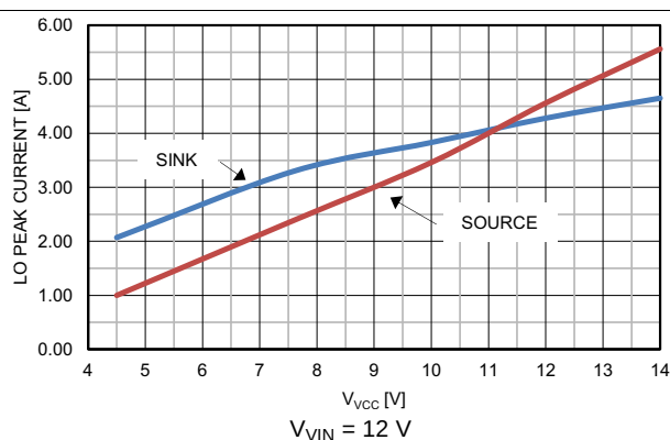
Figure 2. LO Peak Current vs V_{VCC}
