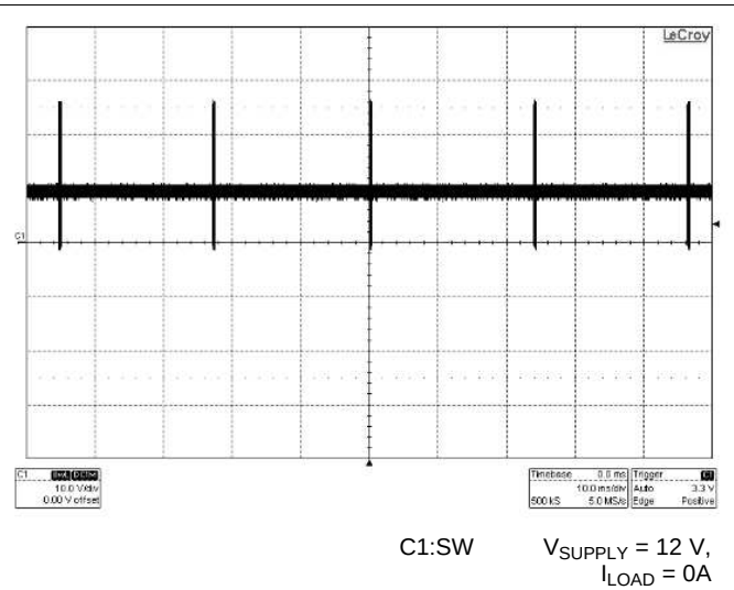
Figure 45. Skip Cycle
