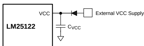
Figure 17. External Bias Supply when 9 V < V_{\text{EXT}} < 14.5 V
