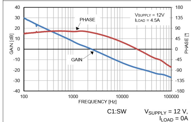
Figure 46. Loop Response
