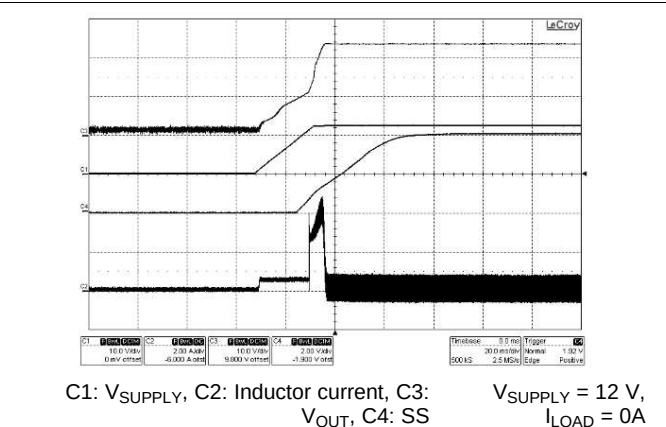
Figure 47. Start-Up
