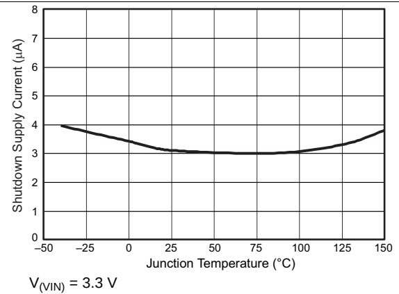
Figure 14. Shutdown Supply Current versus Temperature
