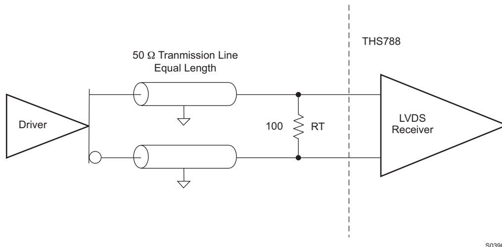
Figure 13. Typical Input Connection to the THS788
