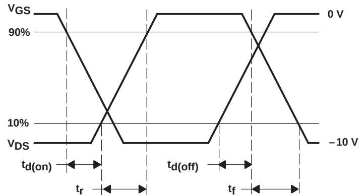
Figure 2. Switching-Time Waveforms
