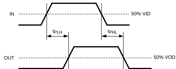
Figure 4. Propagation Delay
