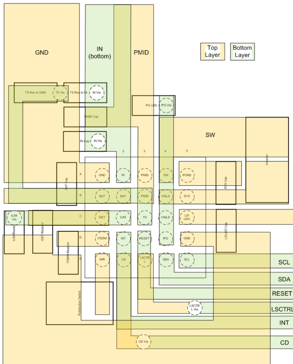
Figure 103. bq25120 Layout
