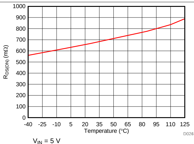
Figure 12. R_{DS(ON)} of High Side MOSFET vs Temperature
