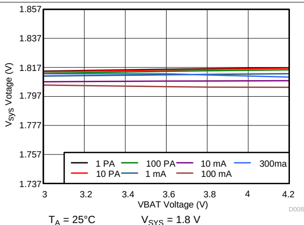
Figure 56. 1.8 V_{SYS} Line Regulation
