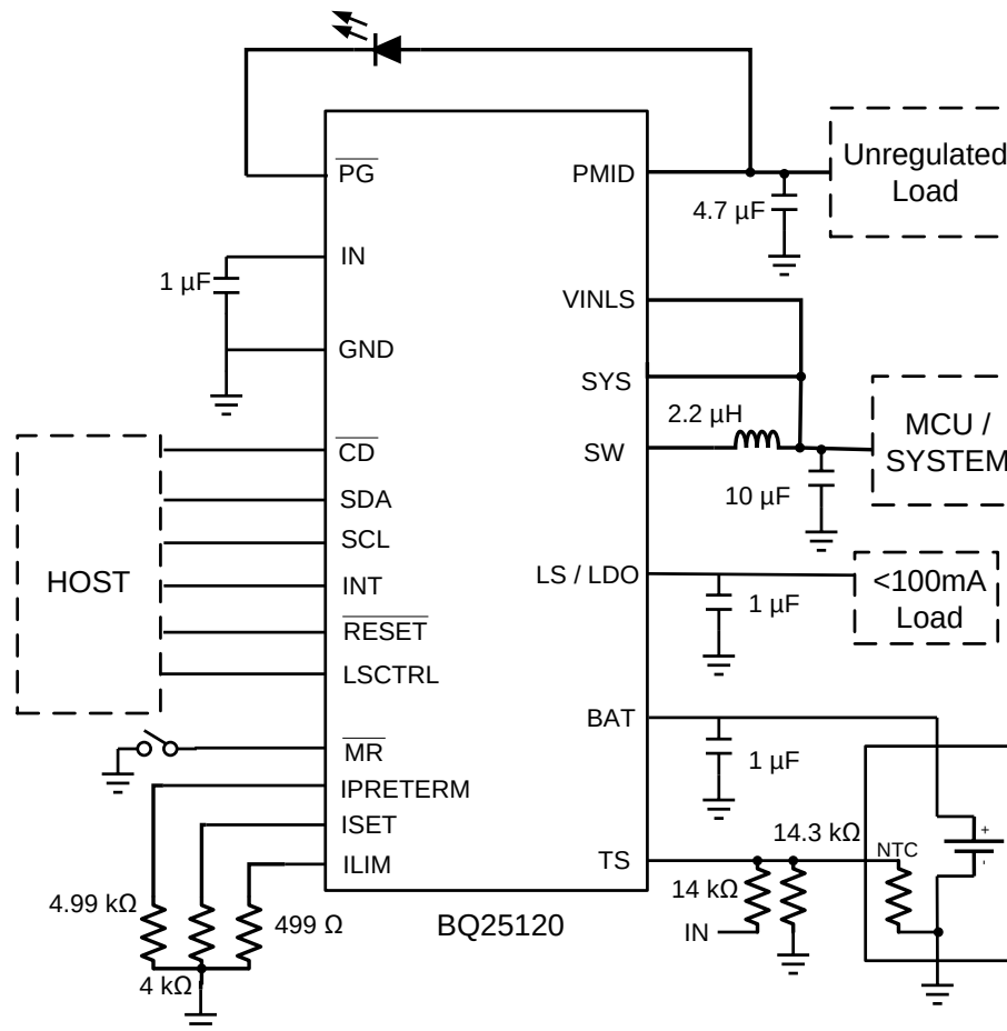
Figure 35. Typical Application Circuit
