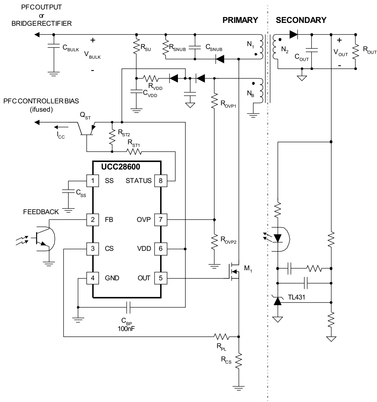
Figure 1. Pin Termination Schematic
