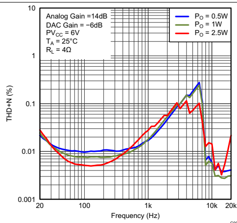
Figure 2. Total Harmonic Distortion + Noise vs Frequency
