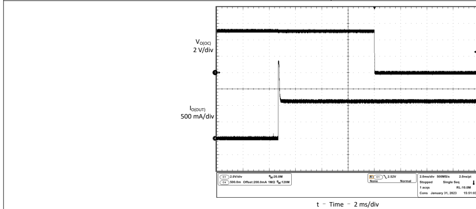
Figure 6-45. 2- \Omega Load Connected to Enabled Device
