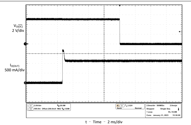
Figure 6-44. 3- \Omega Load Connected to Enabled Device
