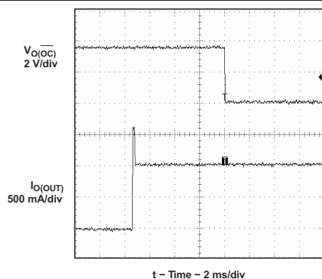
Figure 9-24. 3- \Omega Load Connected to Enabled Device
