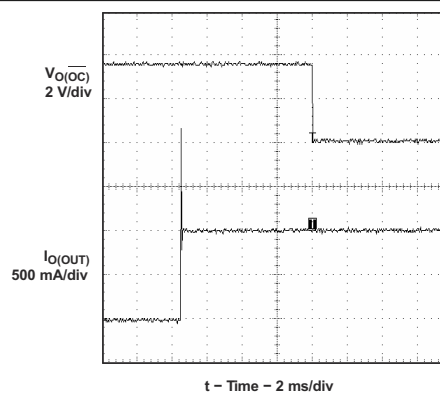
Figure 9-25. 2- \Omega Load Connected to Enabled Device
