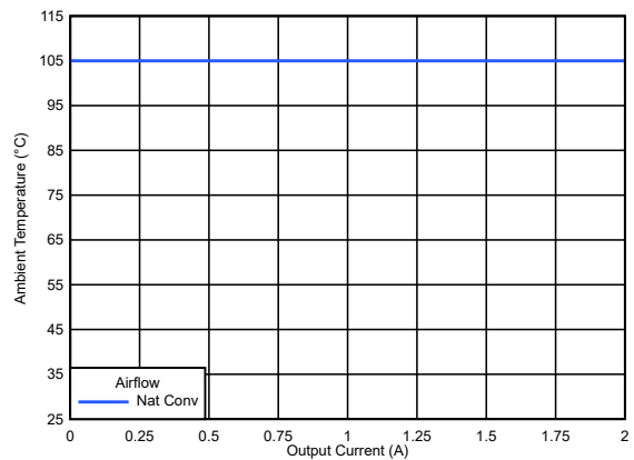
The device is soldered to a 64-mm × 83-mm, 4-layer PCB. Figure 7-10. Safe Operating Area (All V_{OUT} )
