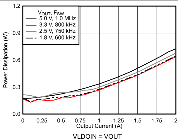
Figure 7-8. Power Dissipation
