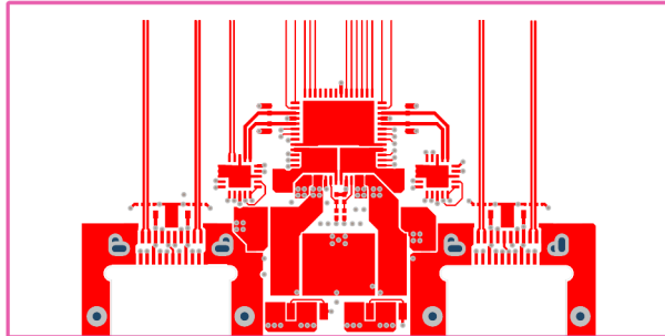
Figure 11-22. SSTXRX1 Layer
