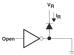
Figure 6-5. I_R Test Circuit
