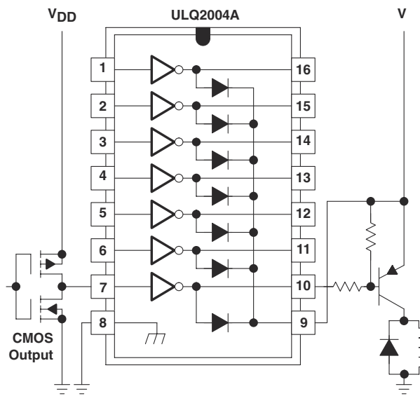
Figure 8-4. Buffer for Higher Current Loads
