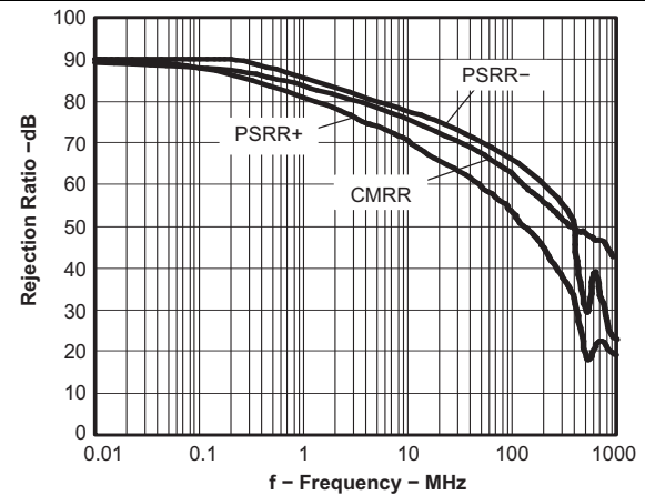
Figure 26. Rejection Ratio vs Frequency
