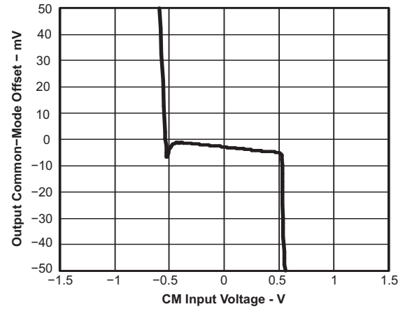
Figure 75. Output Common-Mode Offset vs CM Input Voltage
