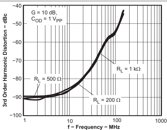
Figure 47. HD3 vs Frequency
