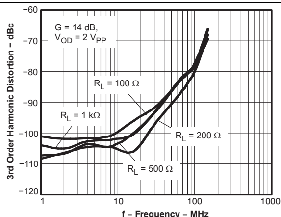
Figure 8. HD3 vs Frequency
