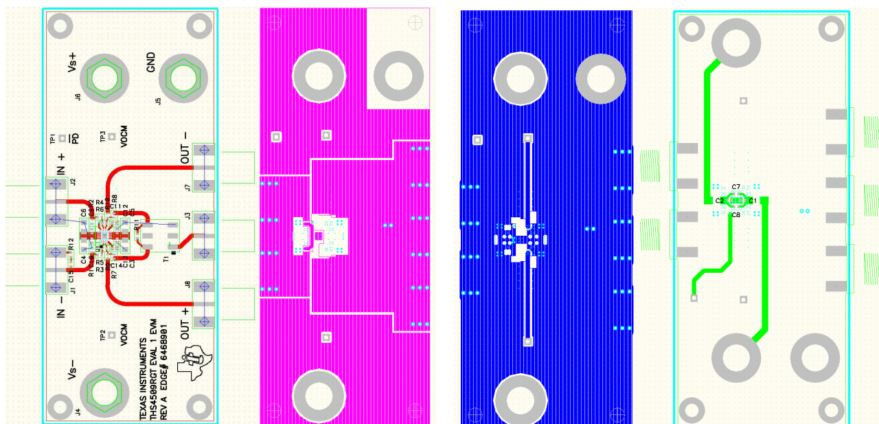
Figure 96. THS4509-Q1 EVAL1 EVM Layer 1 Through 4
