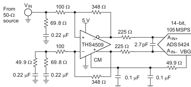
Figure 90. THS4509-Q1 + ADS5424-SP Circuit
