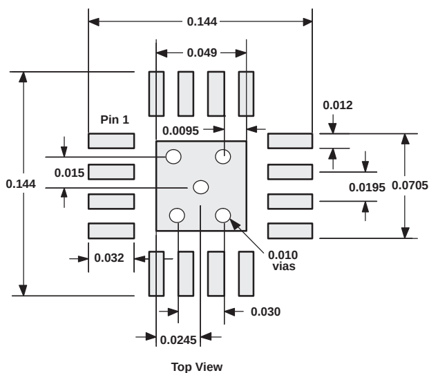
Figure 94. QFN Etch and Via Pattern
