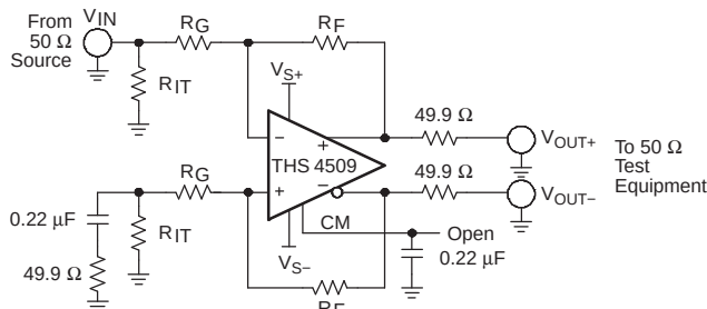
Figure 78. S-Parameter, Sr, Transient Response, Settling Time, Z_o , Overdrive Recovery, V_{OUT} Swing, and Turnon and Turnoff Test Circuit
