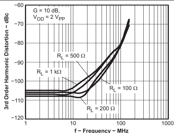
Figure 6. HD3 vs Frequency
