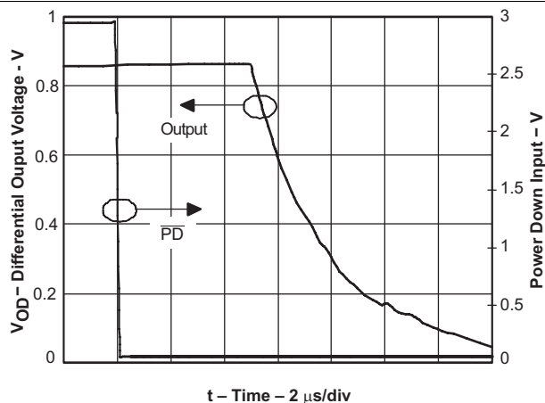
Figure 69. Turn-off Time
