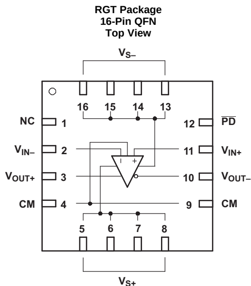
Pin Functions
