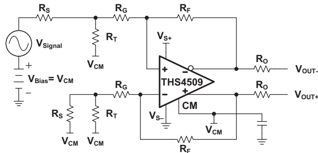
Figure 84. THS4509-Q1 DC-Coupled Single Supply With Input Biased to V_{CM}
