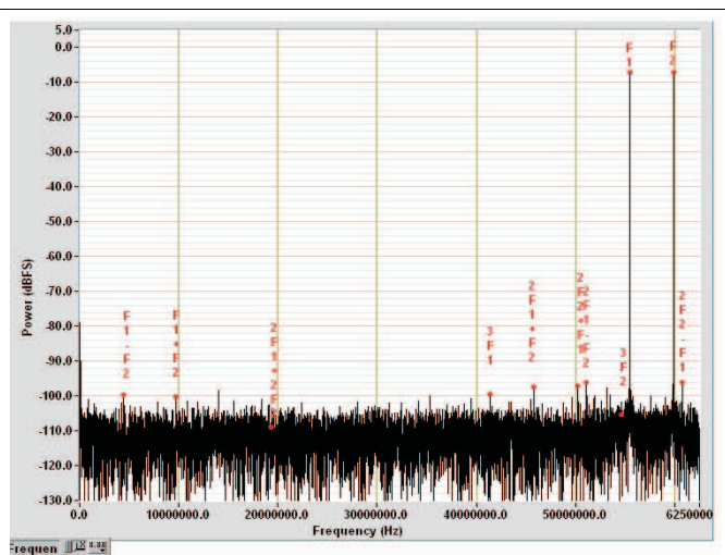
Figure 89. THS4509-Q1 + ADS5500-EP Two-Tone Fft With 65-MHz and 70-MHz Input
