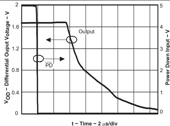
Figure 30. Turnoff Time
