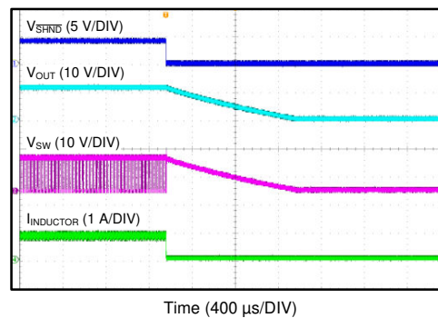
Figure 8-5. Shutdown Waveform ( V_{IN} = 18\text{ V} , V_{OUT} = 12\text{ V} , I_{Load} = 800\text{ mA} )
