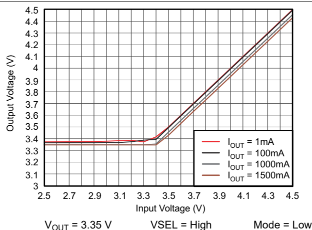
Figure 10-11. TPS61281D DC Output Voltage vs Input Voltage
