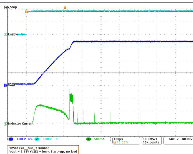
Figure 10-19. Start-Up at No Load
