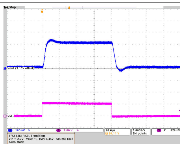
Figure 10-15. TPS61281D Dynamic Voltage Management (VSEL) Load Current 500 mA
