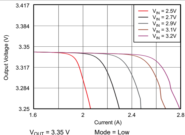
Figure 10-9. TPS61281D DC Output Voltage vs Output Current
