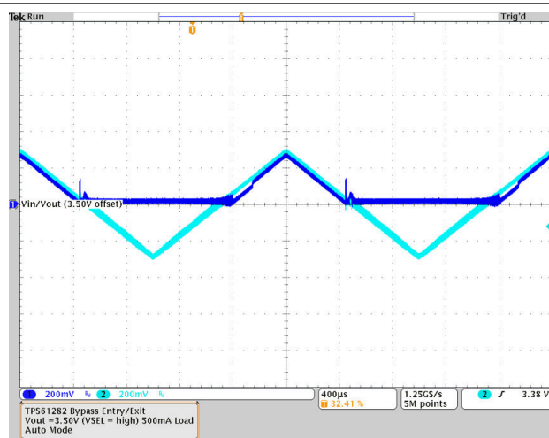
Figure 10-13. Boost to Pass-Through Mode Exit / Entry
