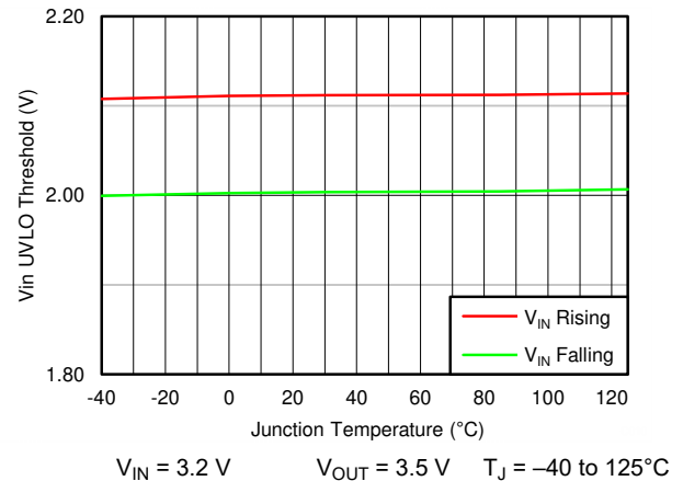
Figure 8-12. V_{IN} UVLO Threshold Rising/Falling vs Junction Temperature
