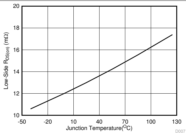
Figure 5-8. Low-Side R_{DS(on)} vs Junction Temperature
