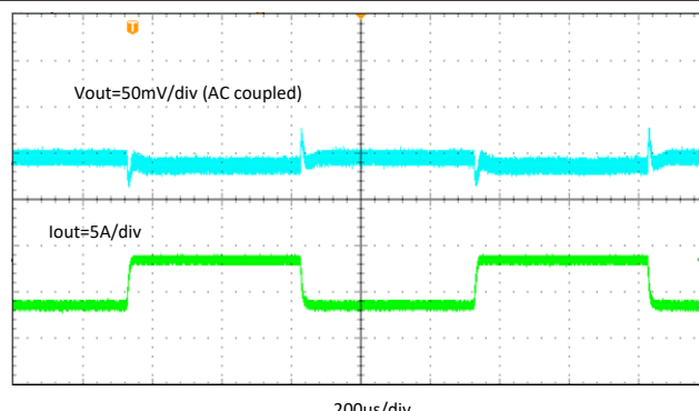
0.6 A to 5.4 A Slew Rate = 2.5 A/μs Figure 7-19. TPS566231 Transient Response
