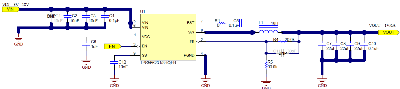
Figure 7-1. 1-V, 6-A Reference Design
