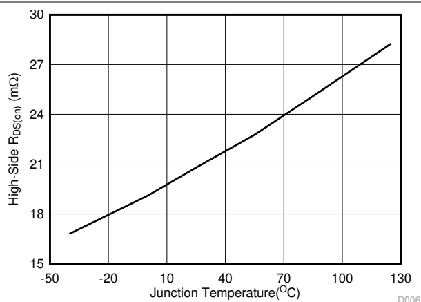
Figure 5-7. High-Side R_{DS(on)} vs Junction Temperature
