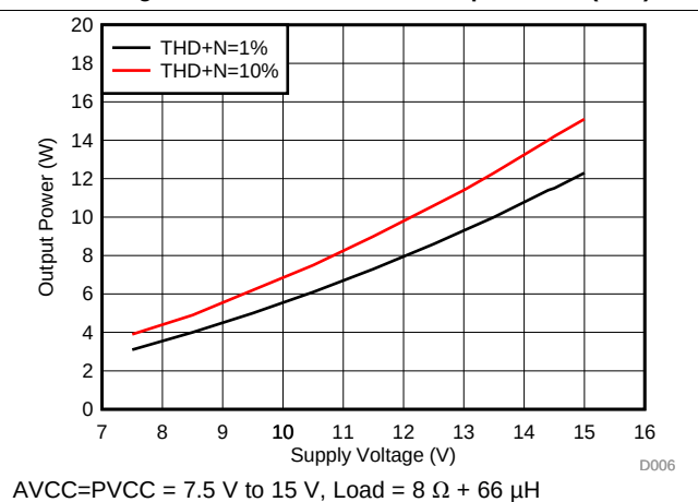
Figure 6. Output Power vs Supply Voltage (BTL)
