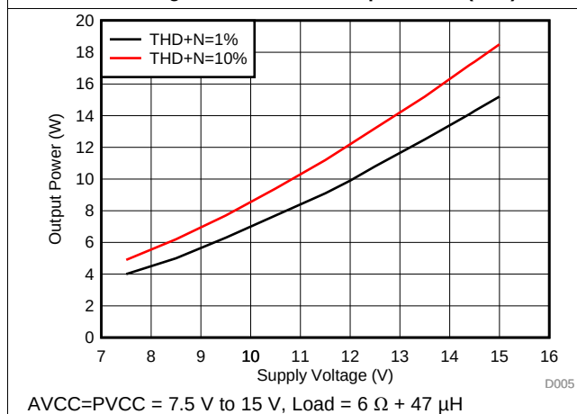
Figure 5. Output Power vs Supply Voltage (BTL)
