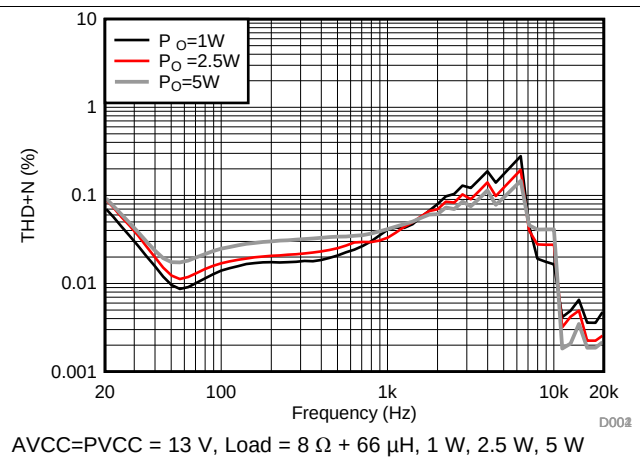
Figure 2. THD+N vs Frequency (BTL)
