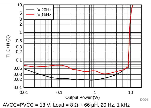
Figure 4. THD+N + Noise vs Output Power (BTL)
