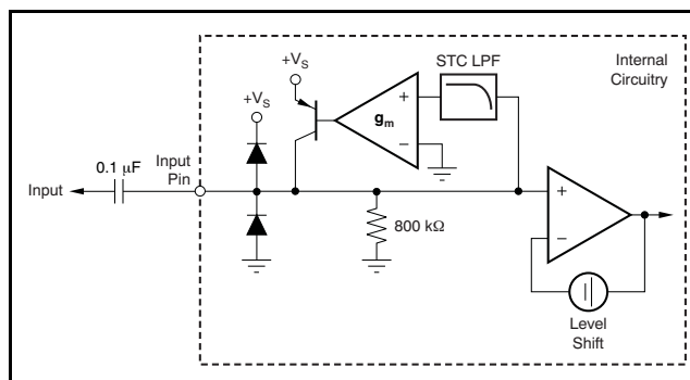
Figure 79. Equivalent AC Sync-Tip-Clamp Input Circuit
