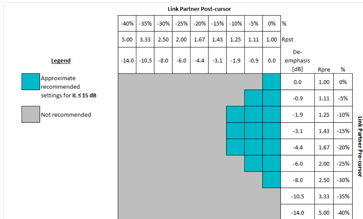
Figure 8-5. Guideline for Link Partner FIR Settings When IL ≤ 15 dB
