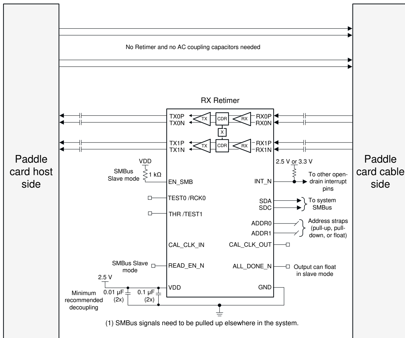
Figure 9-8. Half-Active Cable Application Schematic
