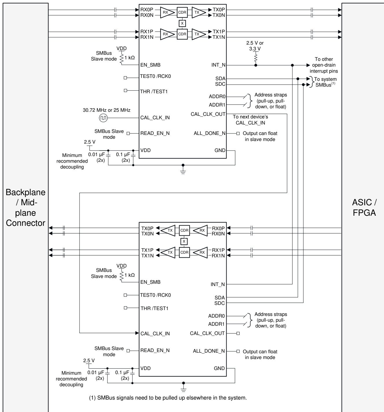
Figure 9-11. Backplane/Mid-Plane Application Schematic
