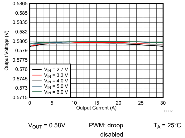
Figure 10-3. Output Voltage Versus Output Current
