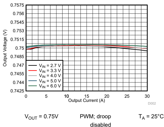
Figure 10-6. Output Voltage Versus Output Current
