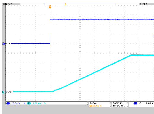
Figure 10-14. Start-Up Timing
