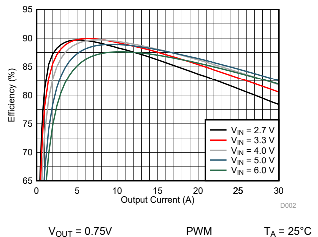
Figure 10-5. Efficiency Versus Output Current
