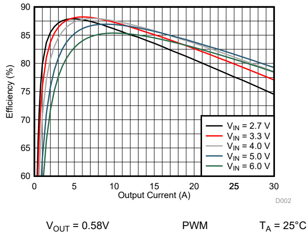
Figure 10-2. Efficiency Versus Output Current
