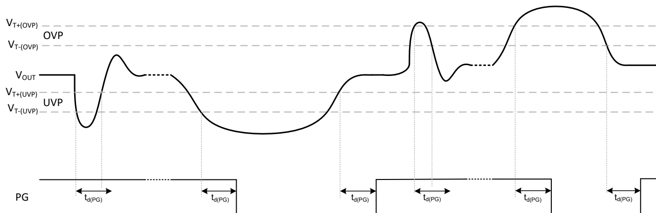
Figure 8-13. PG Timing
