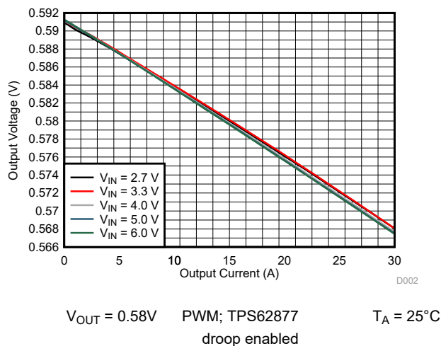
Figure 10-4. Output Voltage Versus Output Current
