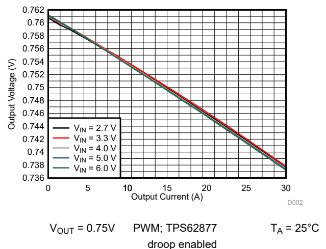
Figure 10-7. Output Voltage Versus Output Current
