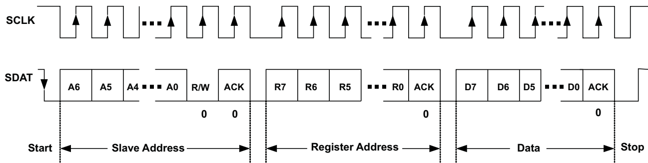
Figure 29. Start and Stop Conditions
