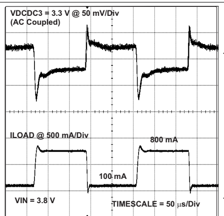
Figure 15. VDCDC3 Load Transient Response
