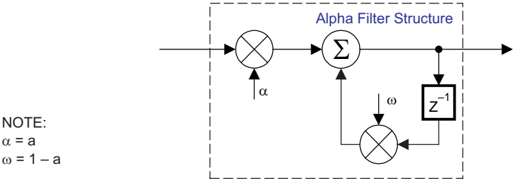
Figure 45. DRC Structure
