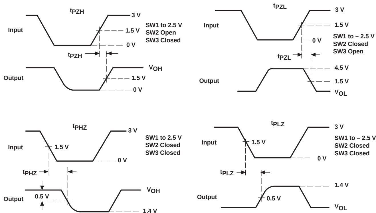
VOLTAGE WAVEFORMS
