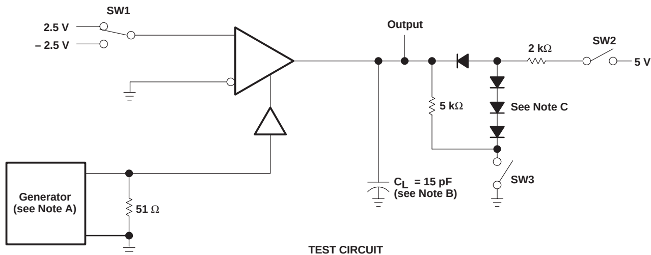
TEST CIRCUIT
