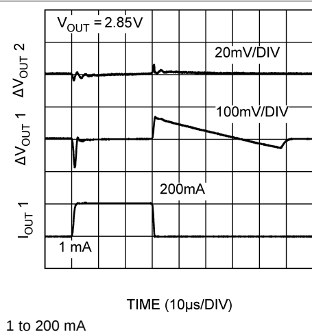
Figure 13. OUT1 Load Transient
