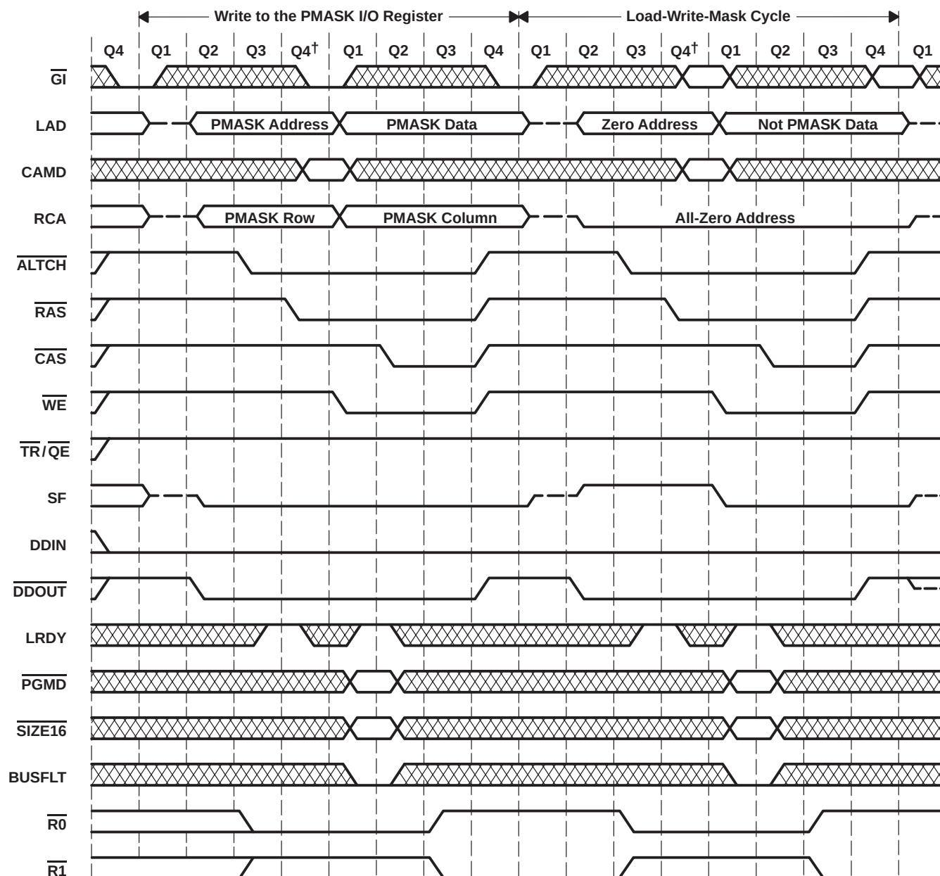
Figure 16. Load-Write-Mask-Cycle Timing
