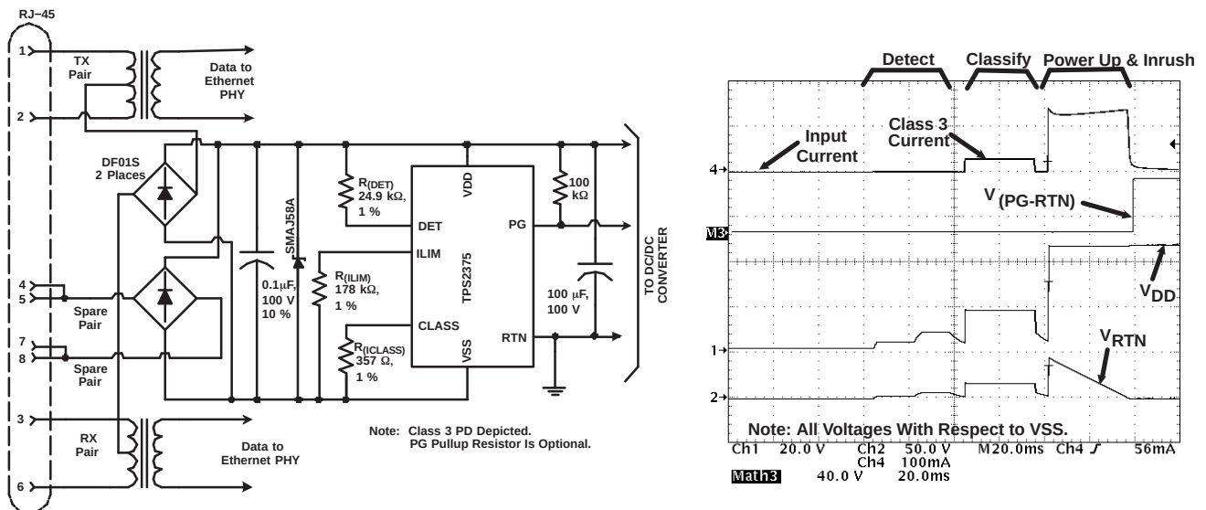
Figure 1. Typical Application Circuit and Startup Waveforms
