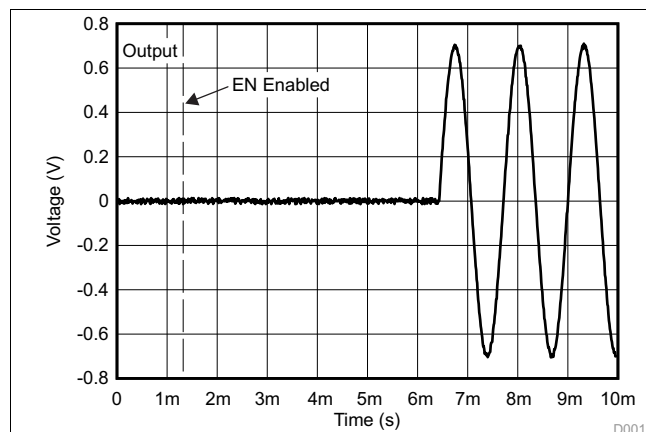
Figure 25. Start-Up Time
