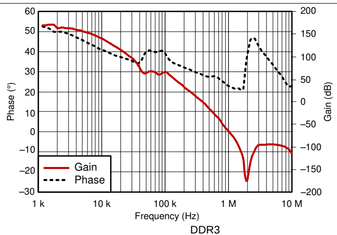
Figure 18. Bode Plot
