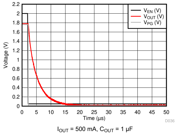
Figure 6-43. LP5912-1.8 V_{OUT} vs V_{EN(OFF)}
