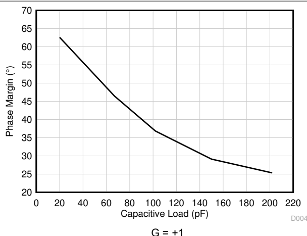
Figure 6-28. Phase Margin vs Capacitive Load
