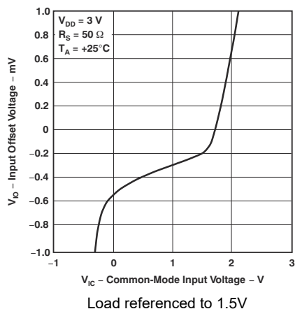
Figure 6-3. Input Offset Voltage vs Common-Mode Input Voltage
