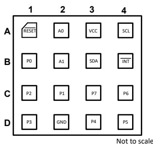
Figure 4-3. DTU (X2QFN) Package, 16-Pin (Top View)
