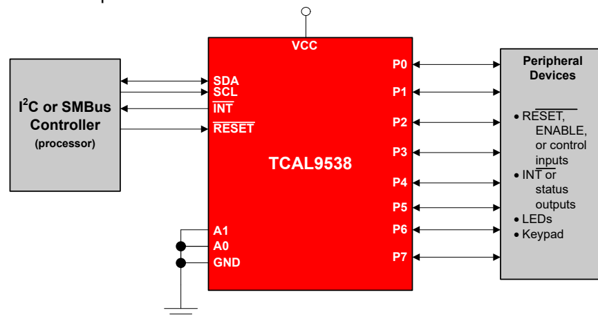
Simplified Schematic
