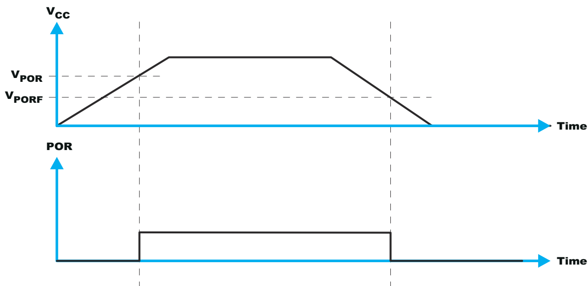
Figure 8-8. V_{POR}
